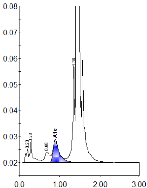
Peak table - ID: 10631890
